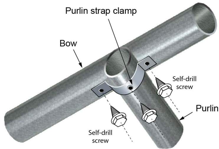
PURLIN END STRAP
