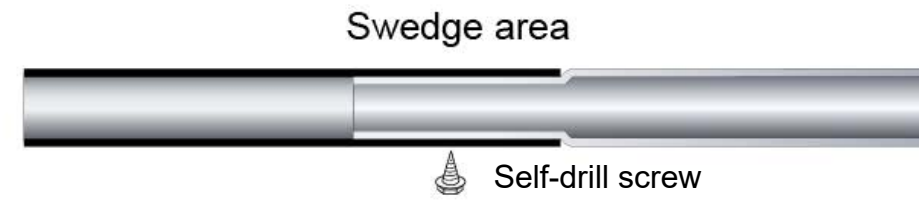
PURLIN SWEDGE DETAIL
